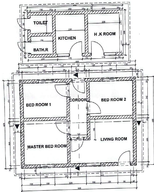
0. Ground Floor (1) 1:50
