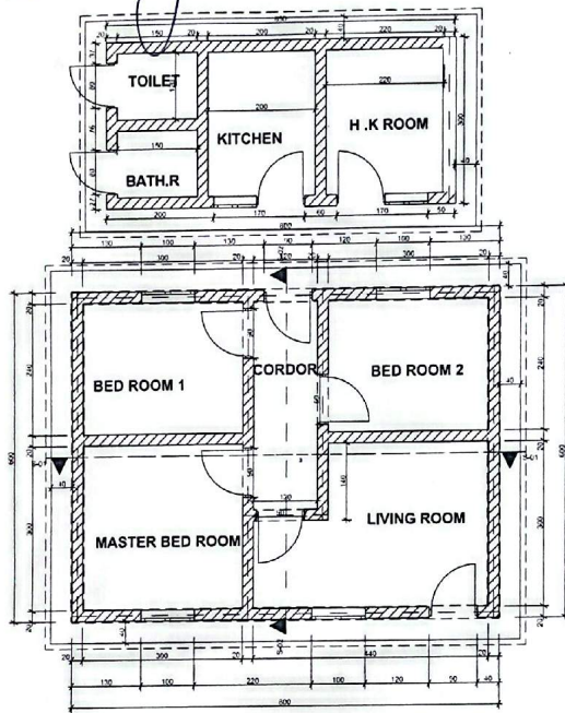
0. Ground Floor (1) 1:50
