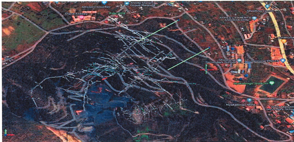
Figure 1. Plan View of the planned drillholes at Nyakabingo (green lines).
