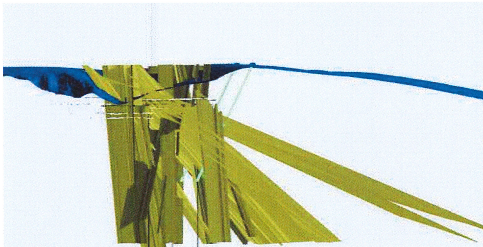
Figure 2. Section view of the planned drillholes at Nyakabingo (green lines)
